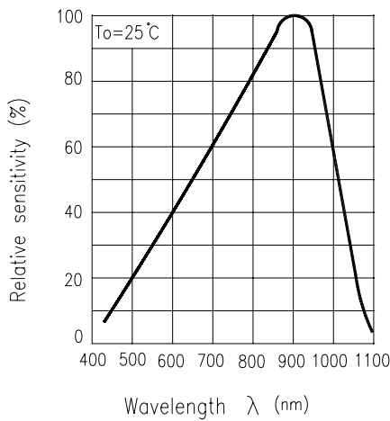
Fig.3 Spectral Sensitivity
